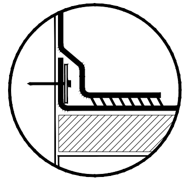
SECUREMENT FASTENED AT BASE OF WALL OR CURB ALTERNATE BASE FASTENING
